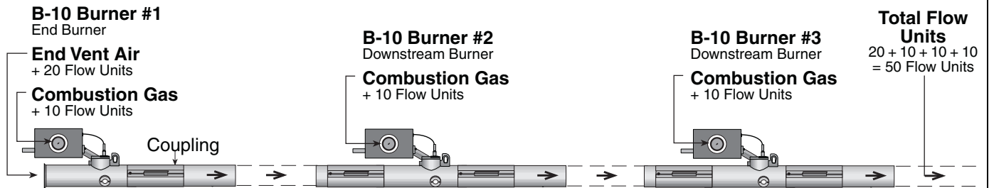
FIGURE 14: Burner Flow Units
